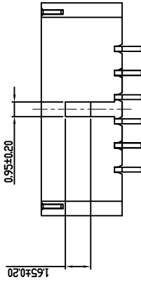
LOCKING WINDOW: ONE PLACE 2 TO 6 PIN
