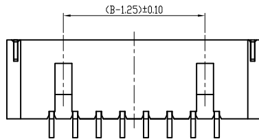
LOCKING WINDOW:TWO PLACE MORE THAN 8 PIN
