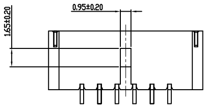
LOCKING WINDOW:ONE PLACE 2 TO 6 PIN
