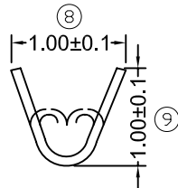
B-B SEC
