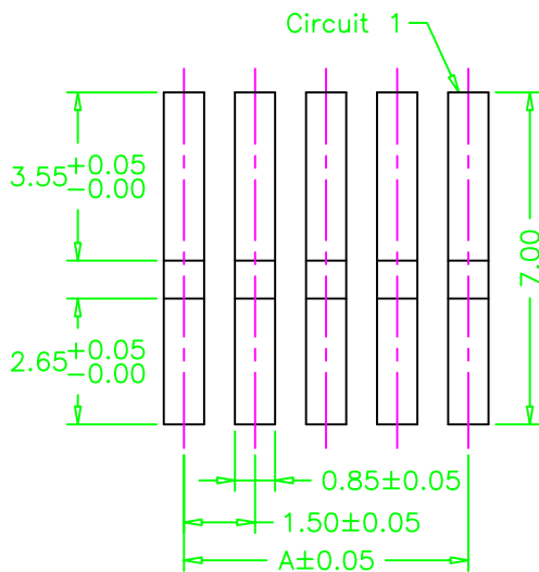
PCB LAYOUT
